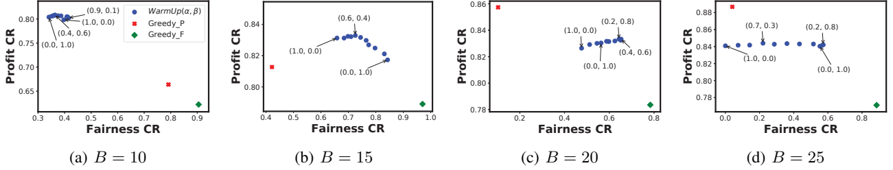
Figure 2: Performance comparisons with Greedy_P and Greedy_F.
