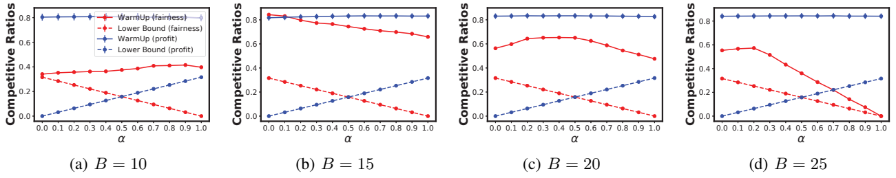
Figure 1: Competitive ratios for profit and fairness with different values of \alpha and \beta with \alpha + \beta = 1 .
